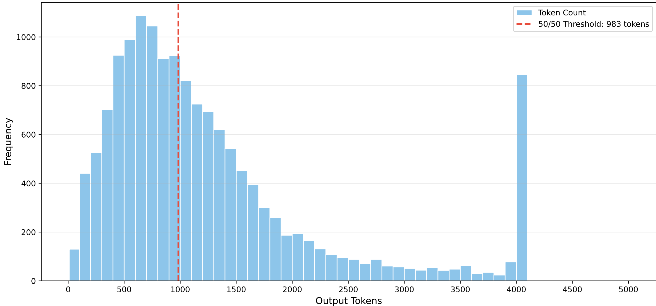
Token Distribution & 50/50 Threshold: DEEPSEEK-8B
