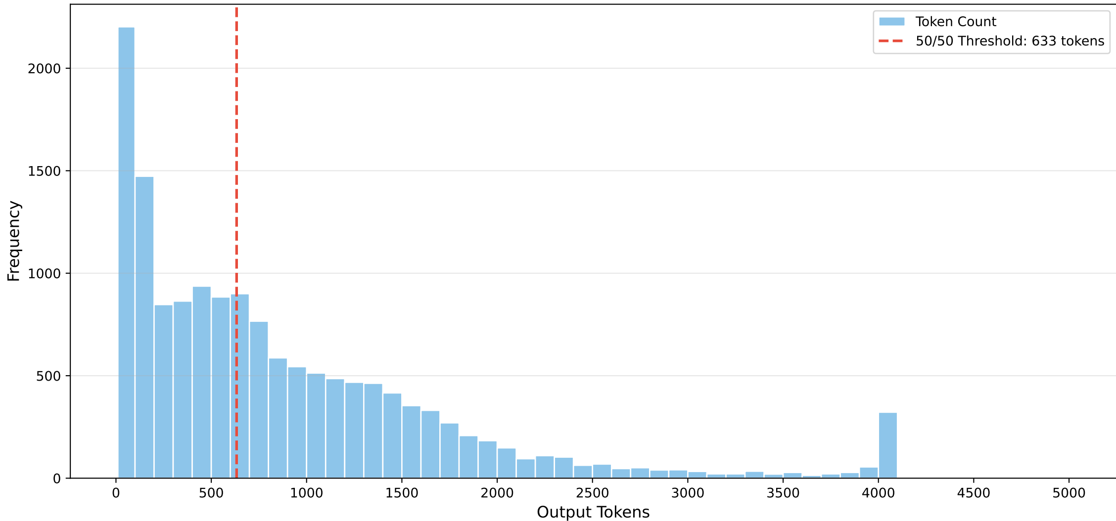
Token Distribution & 50/50 Threshold: DEEPSEEK-R1-QWEN-14B
