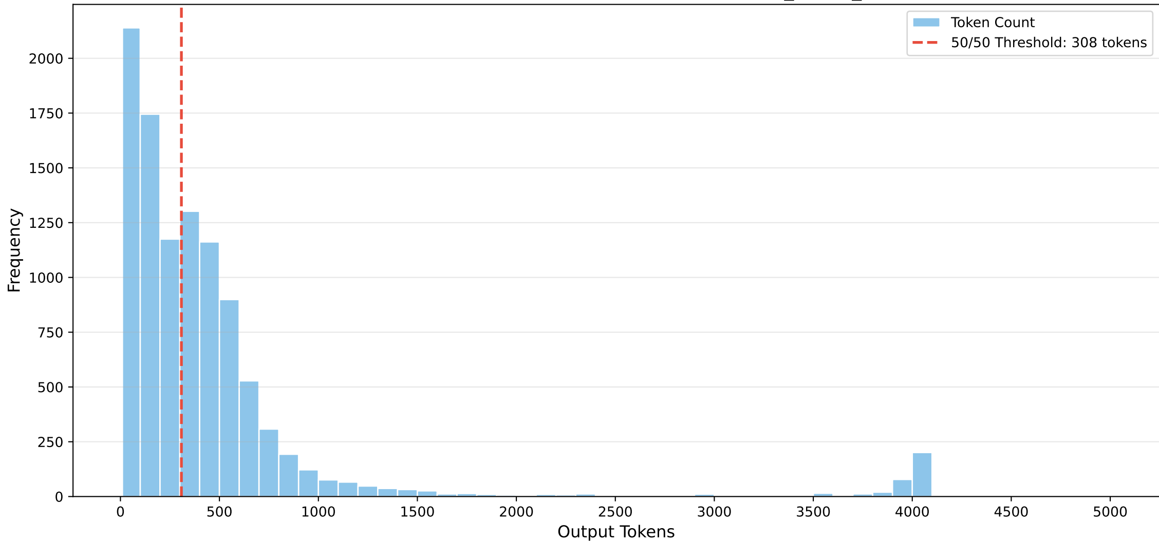
Token Distribution & 50/50 Threshold: MISTRAL_NEMO_12B
