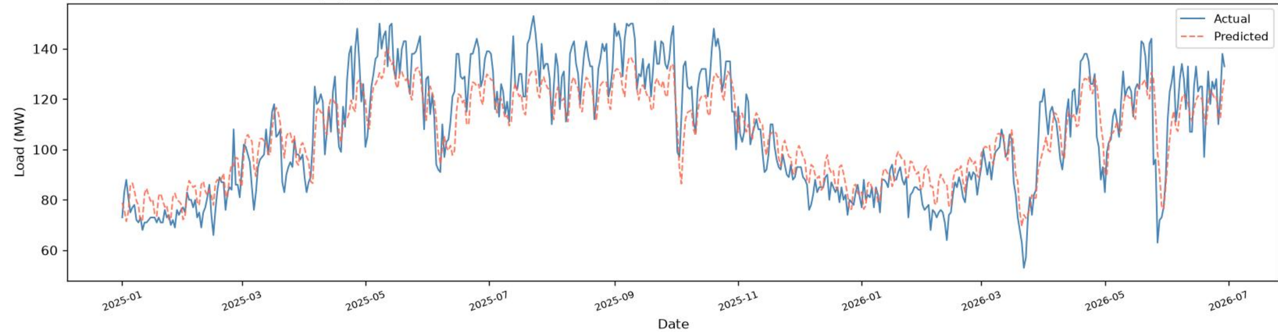
Agargaon | BiGRU+BiLSTM - TEST ( \geq 2025 ), one-day-ahead ( R^2=0.8113 , RMSE=10.34 , MAE=8.51 , n=536 )
