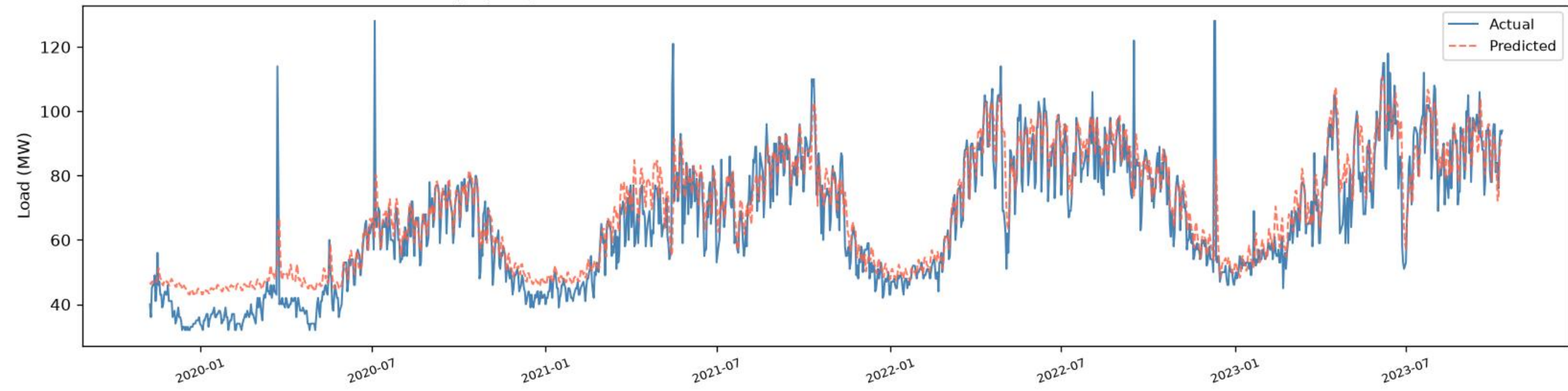
Agargaon | BiGRU+BiLSTM - TRAIN (fit block) ( R^2=0.8343 , RMSE=7.95 , MAE=5.46 , n=1397 )
