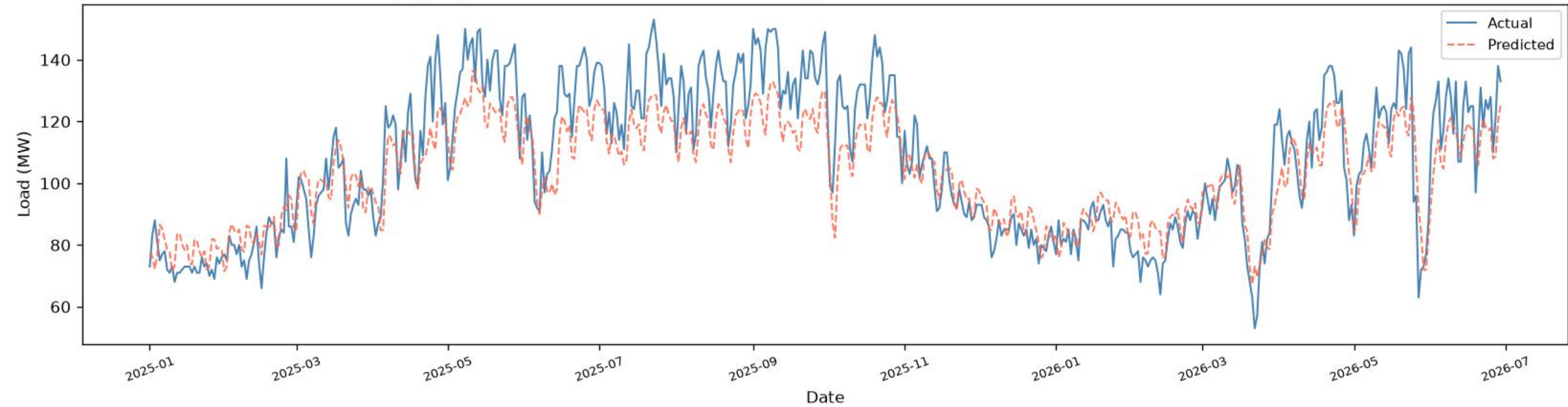
Agargaon | BiLSTM+BiGRU - TEST ( \geq 2025 ), one-day-ahead ( R^2=0.7772 , RMSE=11.23 , MAE=9.14 , n=536 )
