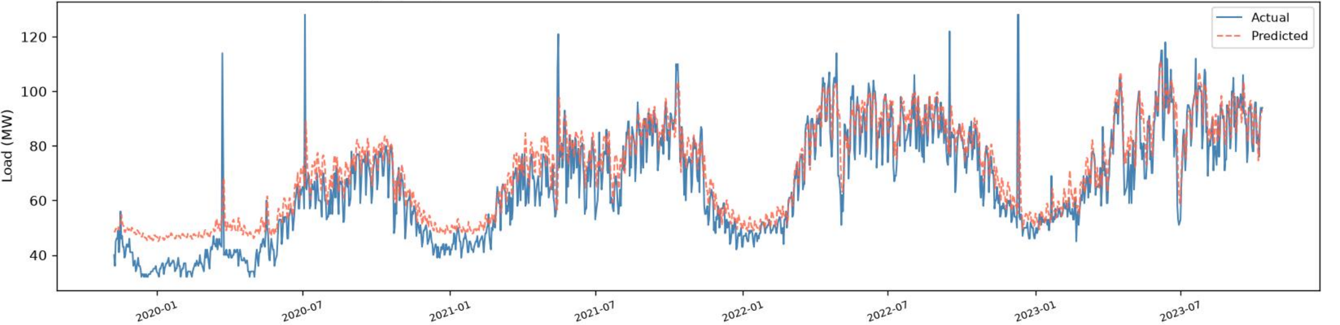
Agargaon | BiLSTM+BiGRU - TRAIN (fit block) (R2=0.8076, RMSE=8.57, MAE=6.38, n=1397)
