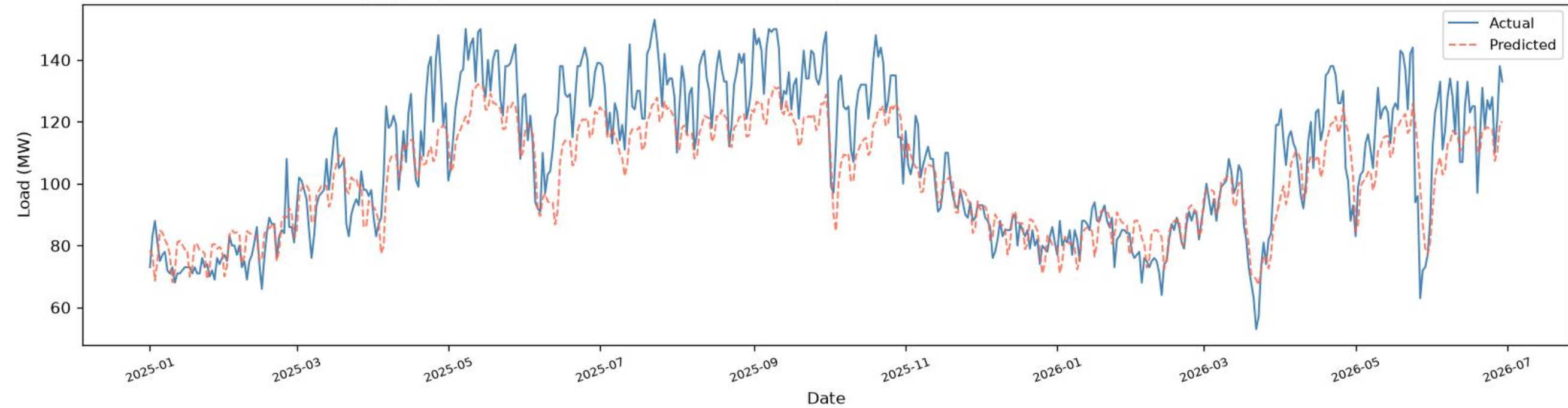
Agargaon | CNN+BiGRU+BiLSTM - TEST ( \geq 2025 ), one-day-ahead ( R^2=0.7381 , RMSE=12.18 , MAE=9.64 , n=536 )
