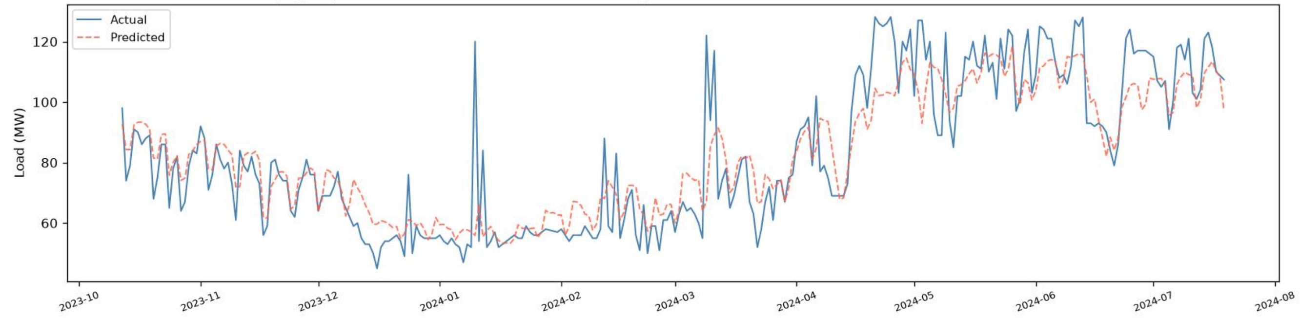
Agargaon | CNN+BiGRU+BiLSTM - VALIDATION (chronological, before test) ( R^2=0.7996 , RMSE=10.90 , MAE=7.80 , n=272 )
