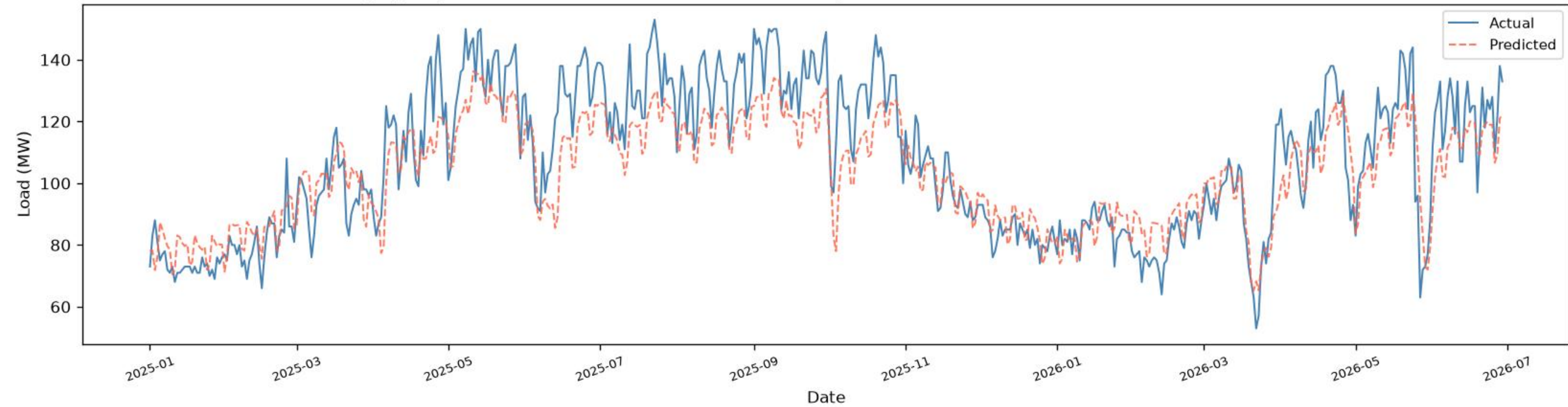
Agargaon | CNN+BiLSTM+BiGRU - TEST ( \geq 2025 ), one-day-ahead ( R^2=0.7593 , RMSE=11.67 , MAE=9.47 , n=536 )
