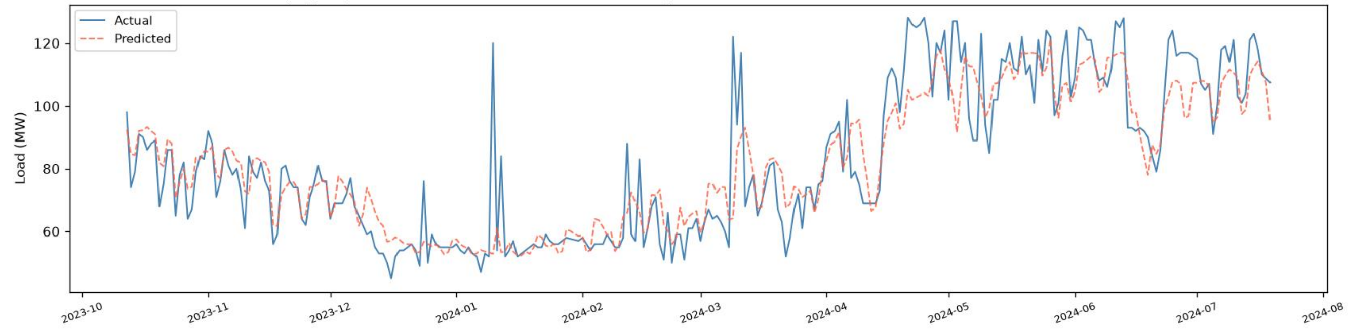
Agargaon | CNN+BiLSTM+BiGRU - VALIDATION (chronological, before test) ( R^2=0.8071 , RMSE=10.69 , MAE=7.17 , n=272 )
