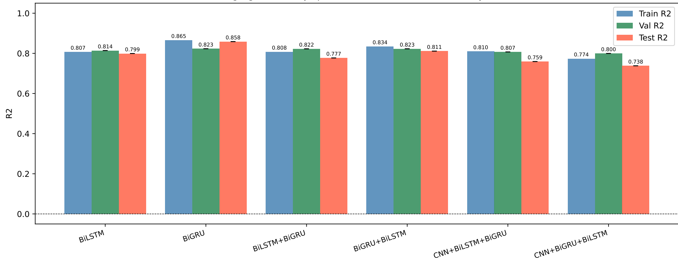
Agargaon - R2 by split (model selection uses VAL only)
