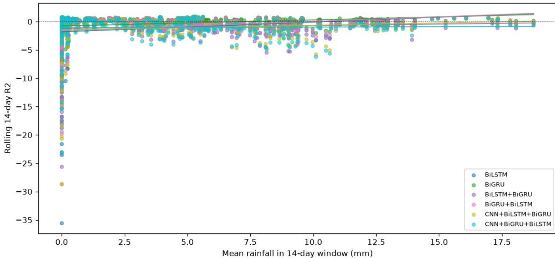
Agargaon - Rain vs R2 (all 6 models, test period)
