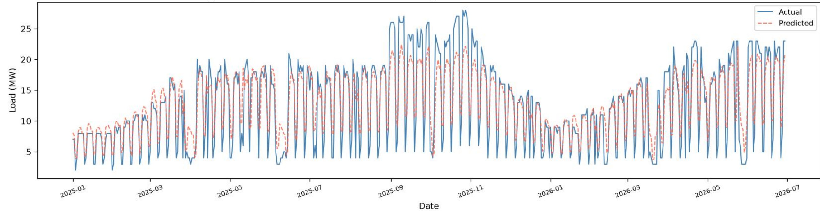
Bangabhaban | BiGRU+BiLSTM - TEST ( \geq 2025 ), one-day-ahead ( R^2=0.7991 , RMSE=3.17 , MAE=2.34 , n=536 )
