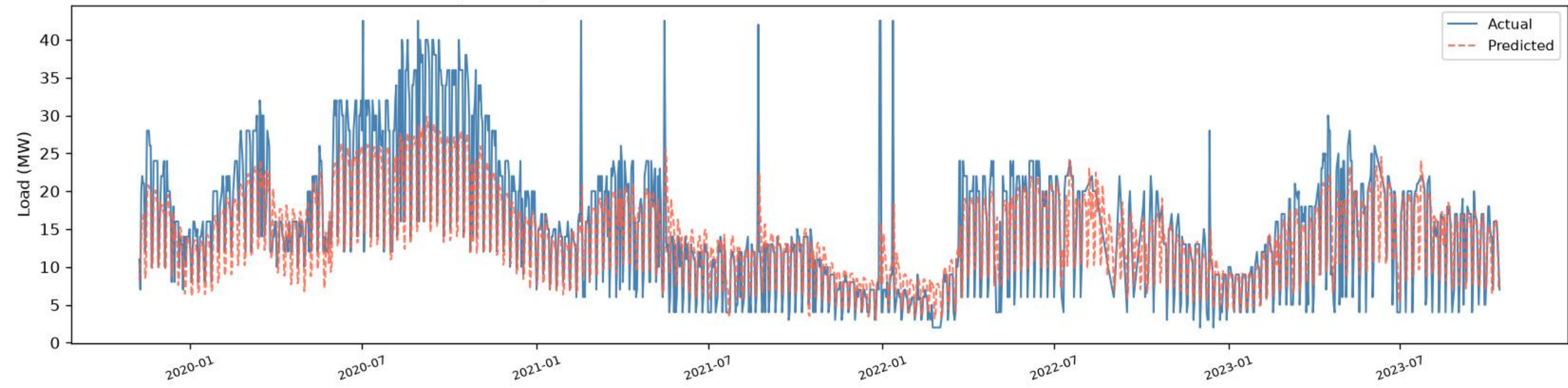
Bangabhaban | BiGRU+BiLSTM - TRAIN (fit block) (R2=0.7215, RMSE=4.67, MAE=3.15, n=1278)
