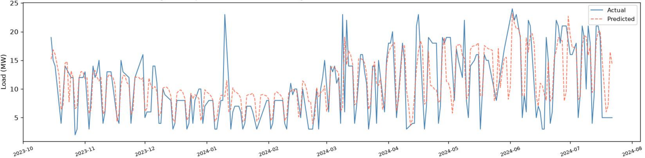
Bangabhaban | BiGRU - VALIDATION (chronological, before test) ( R^2=0.5966 , RMSE=3.79 , MAE=2.60 , n=210 )
