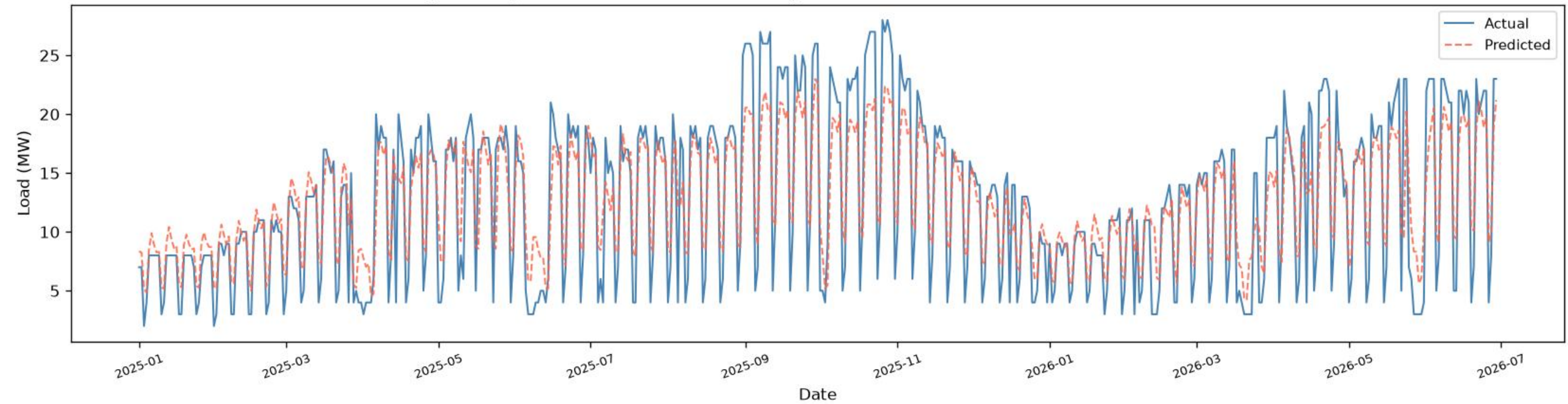
Bangabhaban | BiLSTM - TEST ( \geq 2025 ), one-day-ahead ( R^2=0.7813 , RMSE=3.30 , MAE=2.54 , n=536 )
