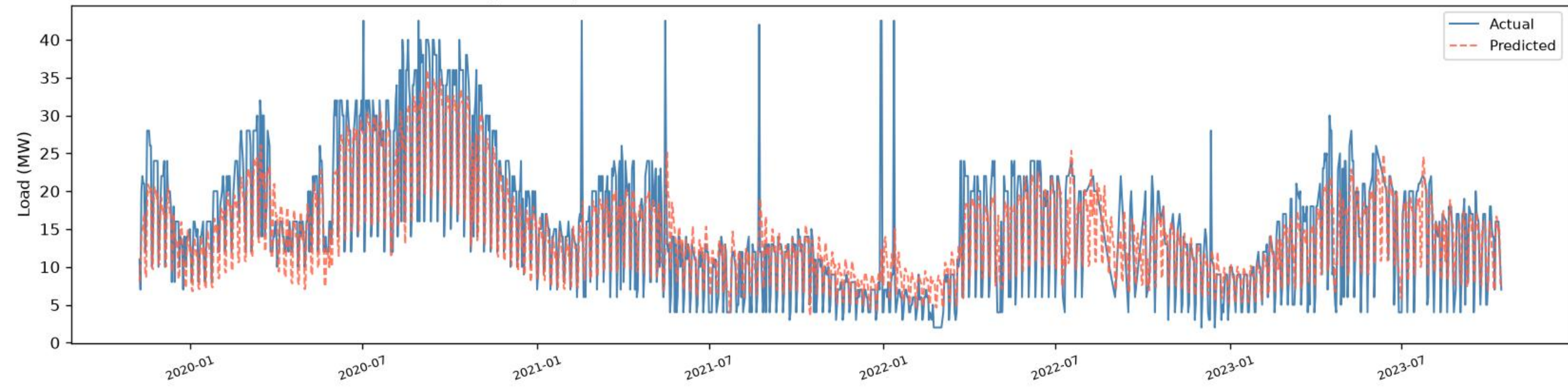
Bangabhaban | BiLSTM - TRAIN (fit block) ( R^2=0.7625 , RMSE=4.31, MAE=2.99, n=1278 )
