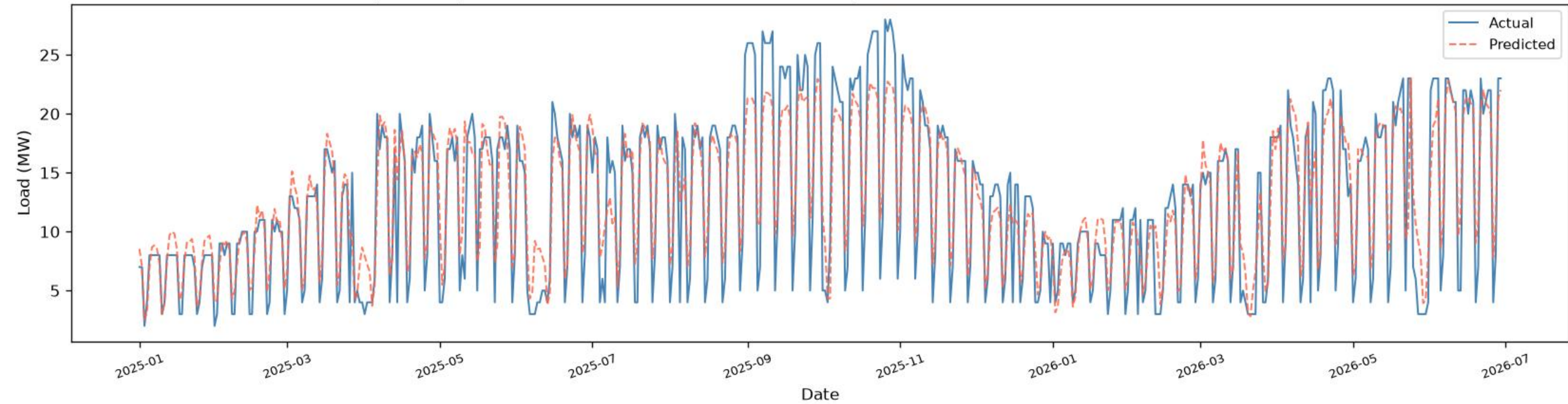
Bangabhaban | CNN+BiGRU+BiLSTM - TEST ( \geq 2025 ), one-day-ahead ( R^2=0.8368 , RMSE=2.85 , MAE=2.16 , n=536 )
