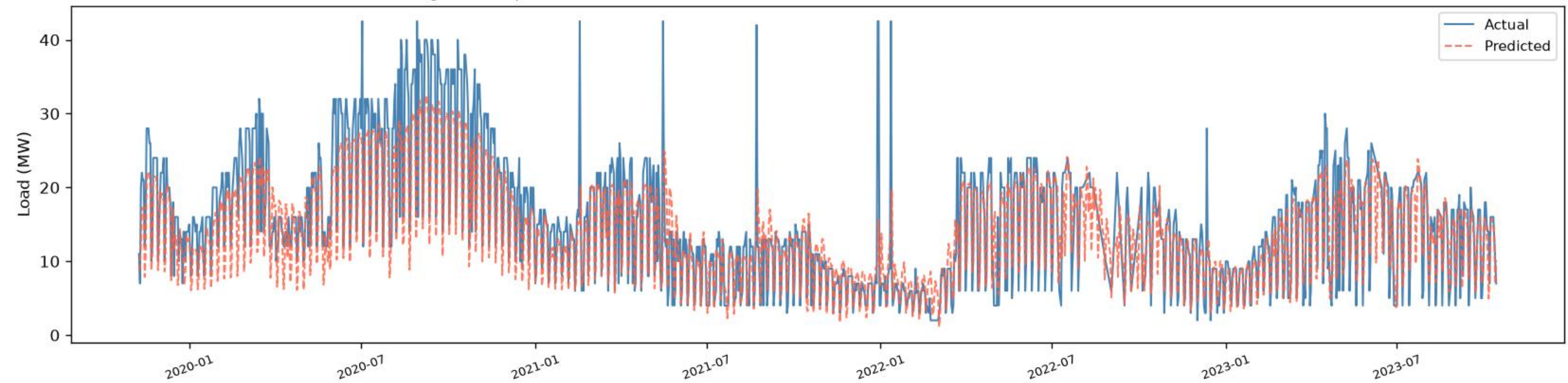
Bangabhaban | CNN+BiGRU+BiLSTM - TRAIN (fit block) (R2=0.7742, RMSE=4.21, MAE=2.83, n=1278)
