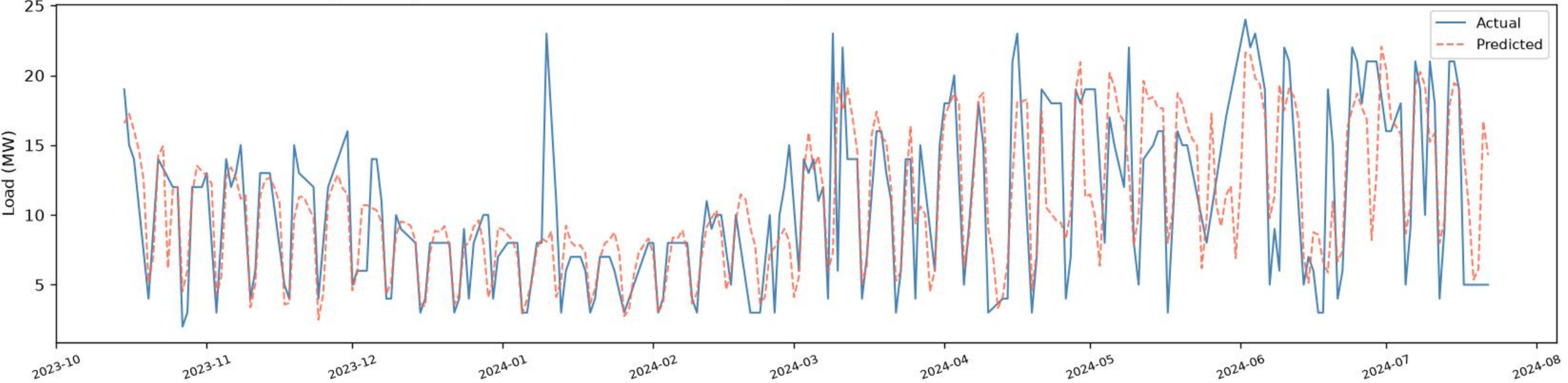
Bangabhaban | CNN+BiGRU+BiLSTM - VALIDATION (chronological, before test) (R2=0.5947, RMSE=3.80, MAE=2.56, n=210)
