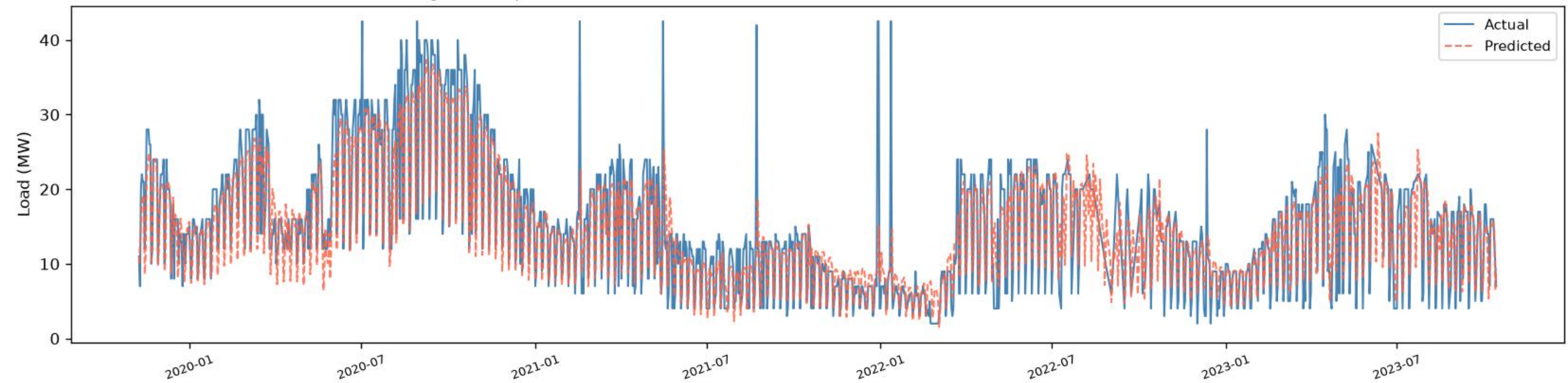
Bangabhaban | CNN+BiLSTM+BiGRU - TRAIN (fit block) (R2=0.8143, RMSE=3.81, MAE=2.40, n=1278)
