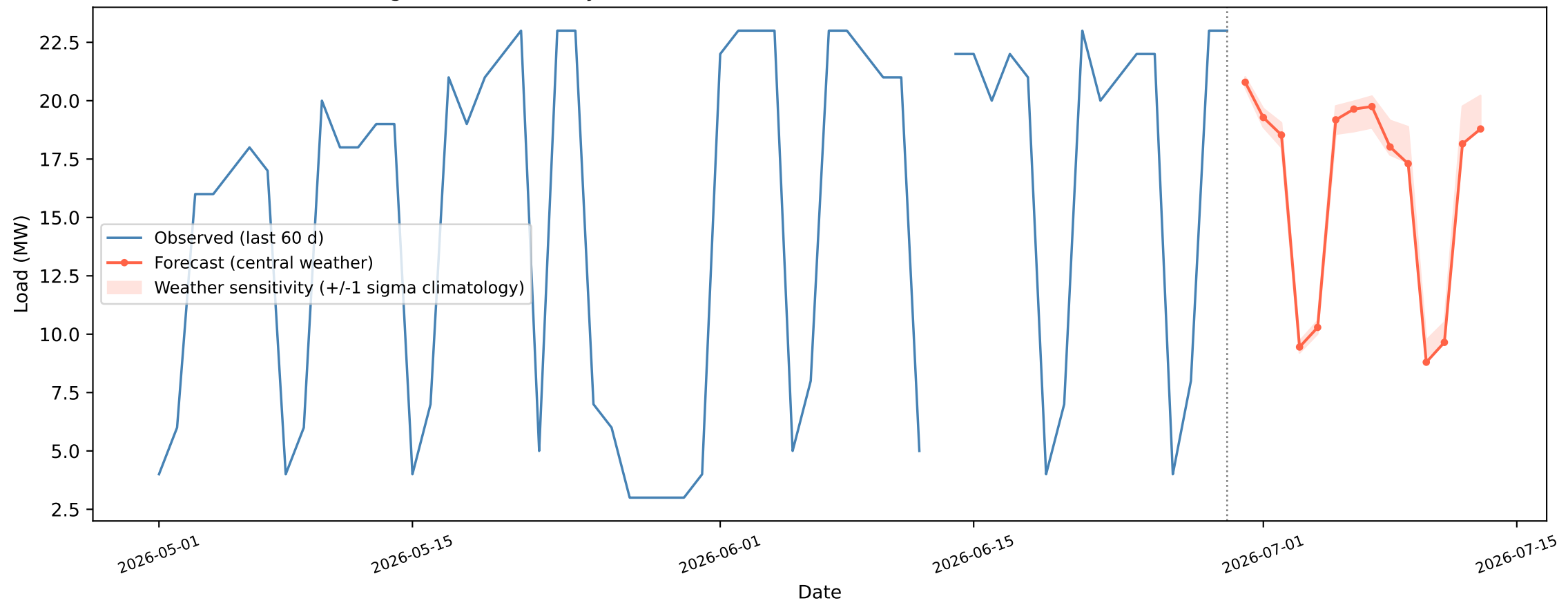
Bangabhaban - 14-day recursive forecast (BiGRU+BiLSTM), weather mode = forecast
