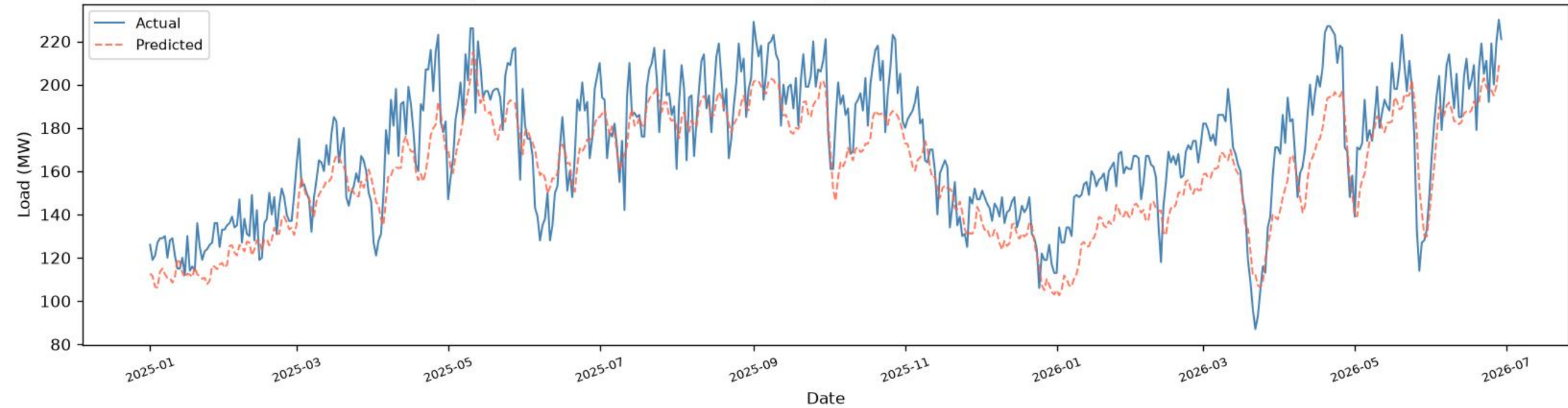
Bashundhara | BiGRU+BiLSTM - TEST ( \geq 2025 ), one-day-ahead ( R^2=0.6511 , RMSE=17.90 , MAE=15.21 , n=536 )
