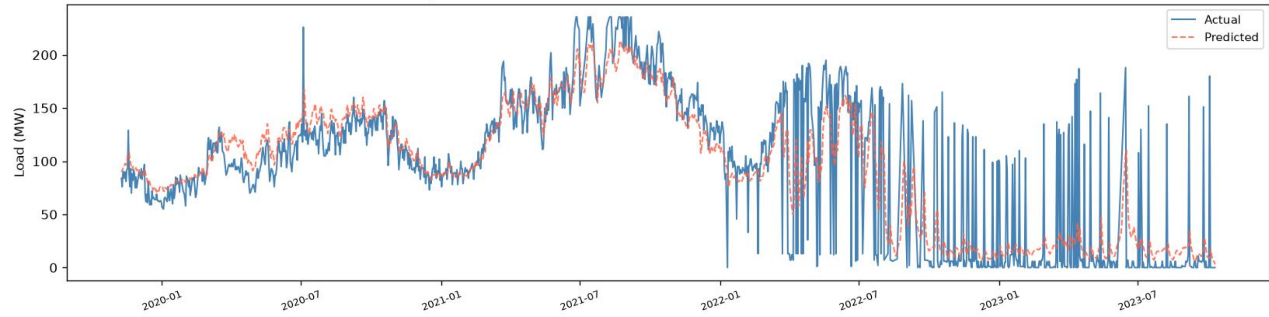
Bashundhara | BiGRU+BiLSTM - TRAIN (fit block) (R2=0.7121, RMSE=34.56, MAE=21.51, n=1289)
