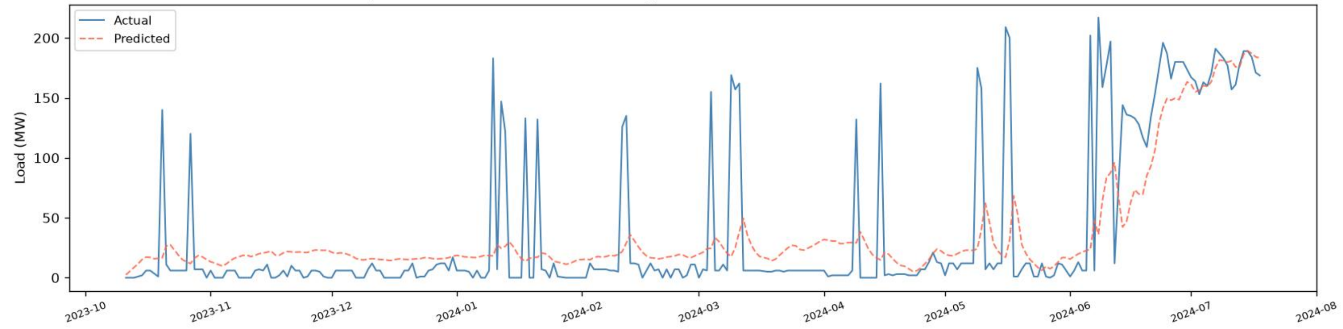
Bashundhara | BiGRU+BiLSTM - VALIDATION (chronological, before test) ( R^2=0.5133 , RMSE=44.95 , MAE=26.70 , n=269 )
