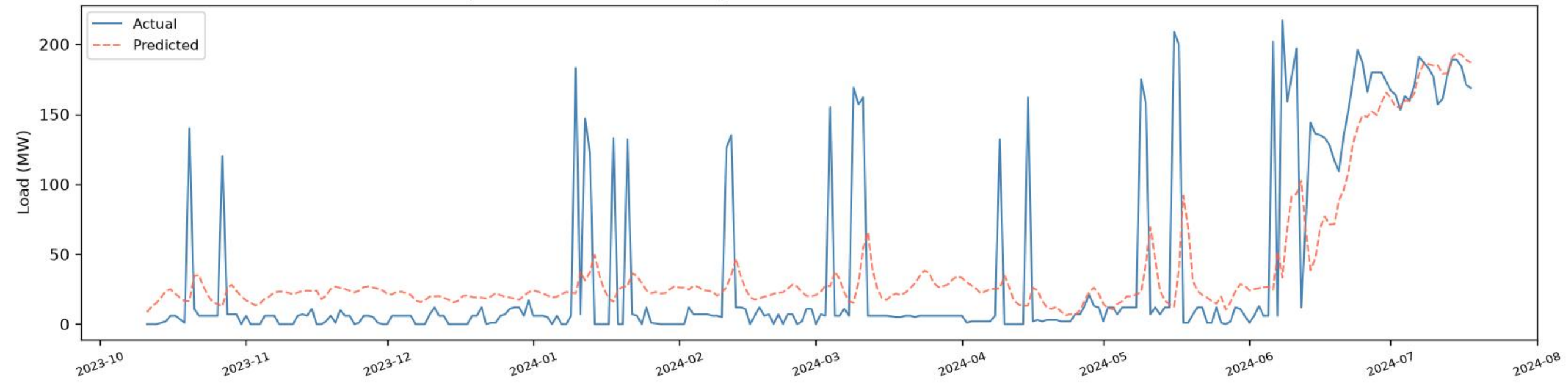
Bashundhara | BiGRU - VALIDATION (chronological, before test) ( R^2=0.4976 , RMSE=45.67, MAE=29.42, n=269)
