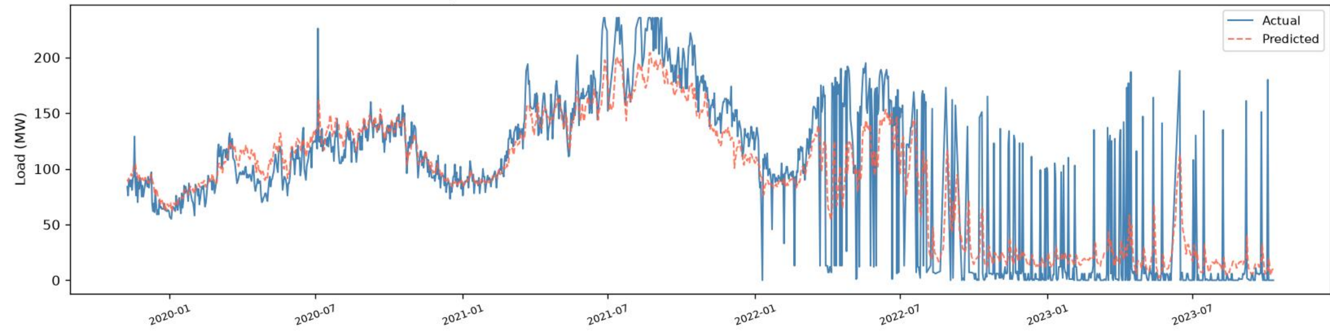
Bashundhara | BiLSTM+BiGRU - TRAIN (fit block) (R2=0.7088, RMSE=34.76, MAE=22.06, n=1289)
