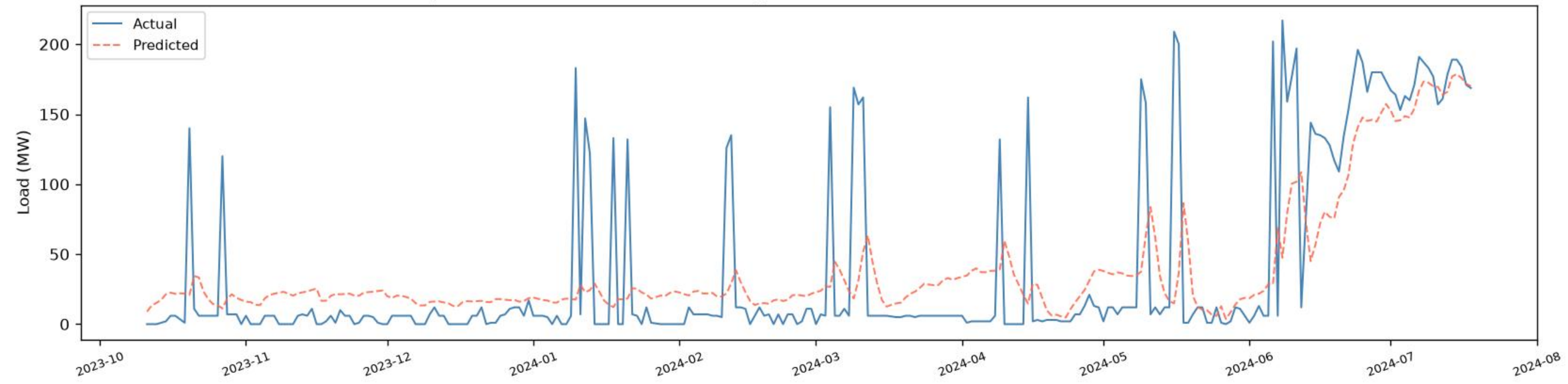
Bashundhara | BiLSTM+BiGRU - VALIDATION (chronological, before test) ( R^2=0.5115 , RMSE=45.03 , MAE=28.94 , n=269 )
