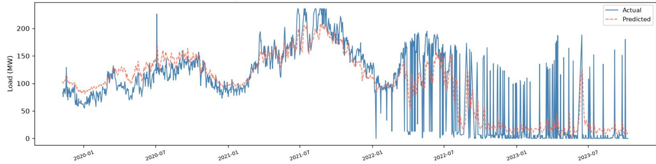
Bashundhara | BiLSTM - TRAIN (fit block) ( R^2=0.6925 , RMSE=35.72 , MAE=23.88 , n=1289 )
