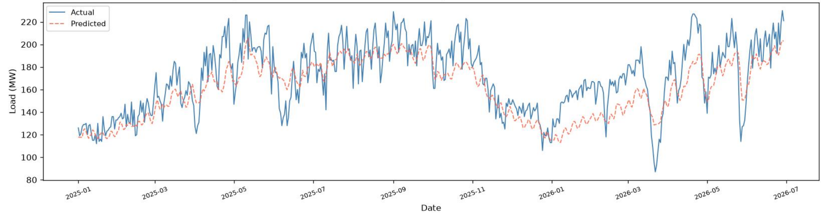
Bashundhara | CNN+BiGRU+BiLSTM - TEST ( \geq 2025 ), one-day-ahead ( R^2=0.5890 , RMSE=19.43 , MAE=16.18 , n=536 )
