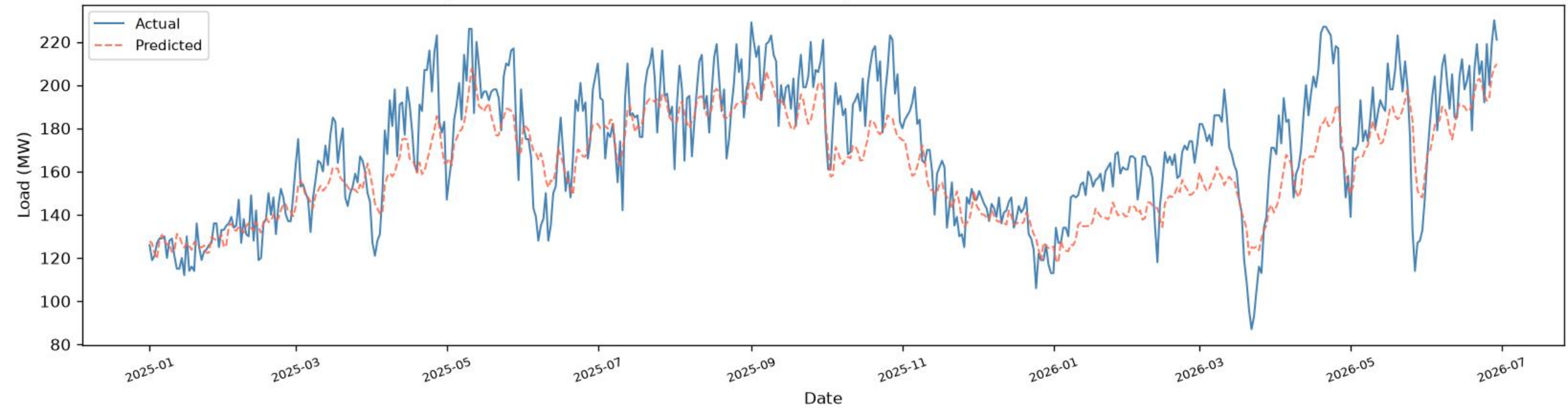
Bashundhara | CNN+BiLSTM+BiGRU - TEST ( \geq 2025 ), one-day-ahead ( R^2=0.6538 , RMSE=17.83 , MAE=14.50 , n=536 )
