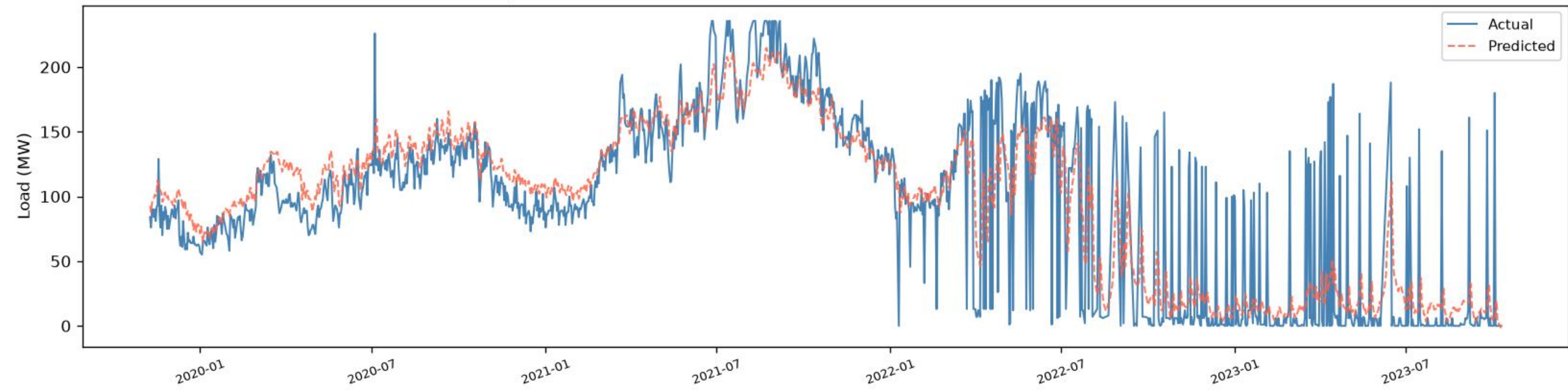
Bashundhara | CNN+BiLSTM+BiGRU - TRAIN (fit block) (R2=0.7103, RMSE=34.67, MAE=21.90, n=1289)
