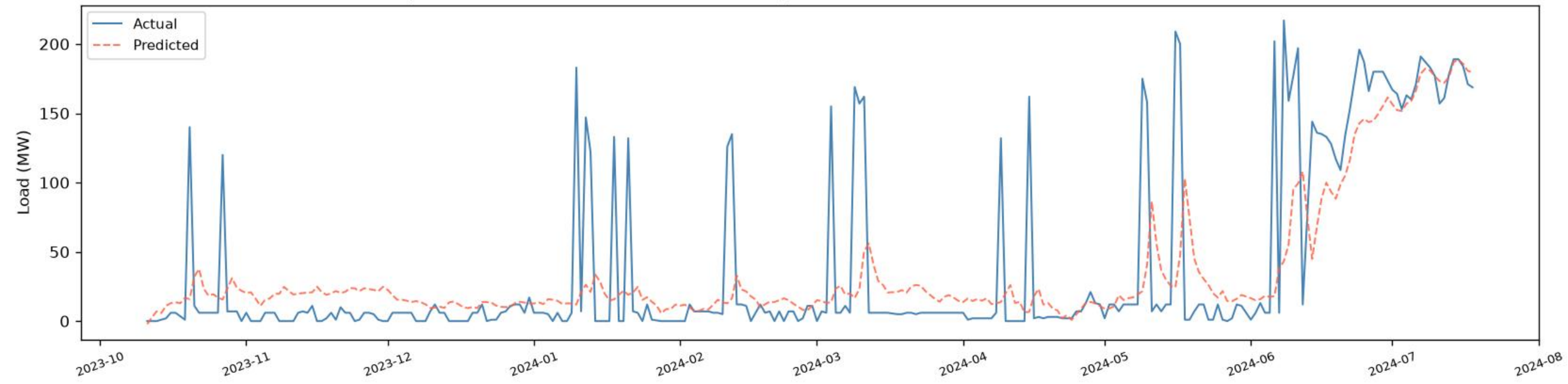
Bashundhara | CNN+BiLSTM+BiGRU - VALIDATION (chronological, before test) ( R^2=0.5181 , RMSE=44.73, MAE=25.12, n=269 )
