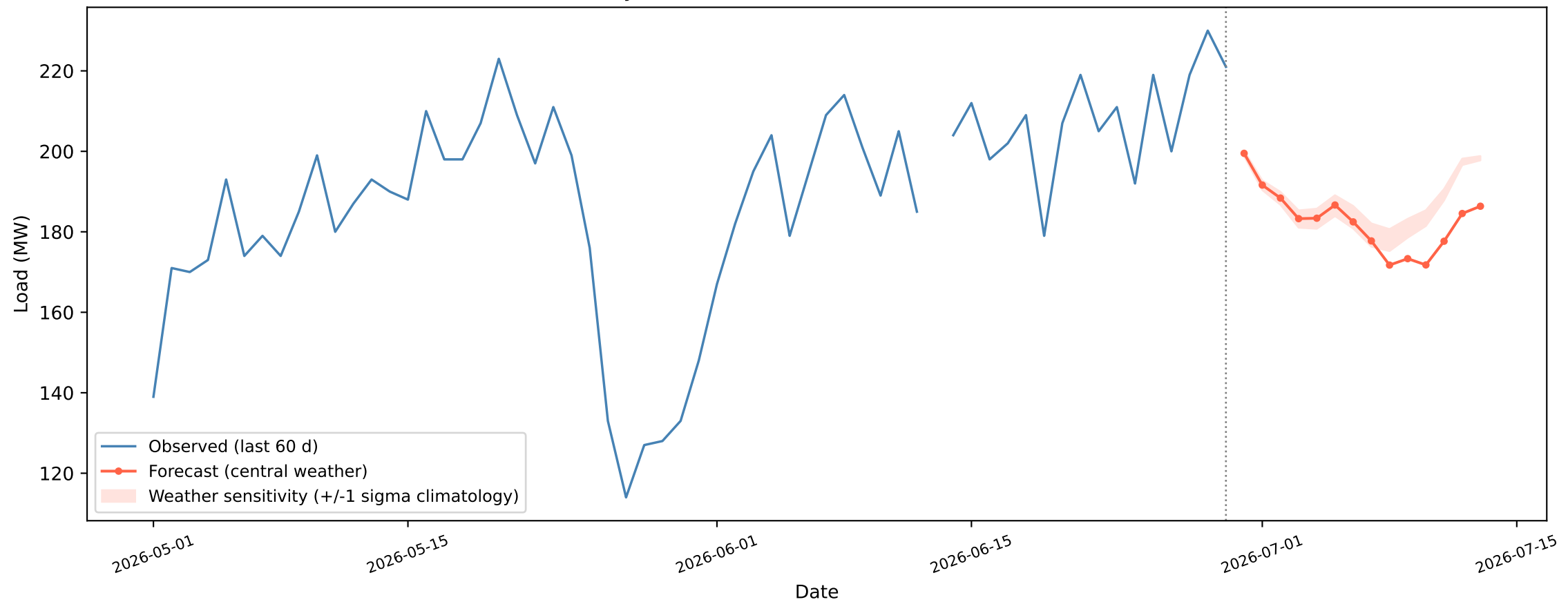
Bashundhara - 14-day recursive forecast (BiLSTM), weather mode = forecast
