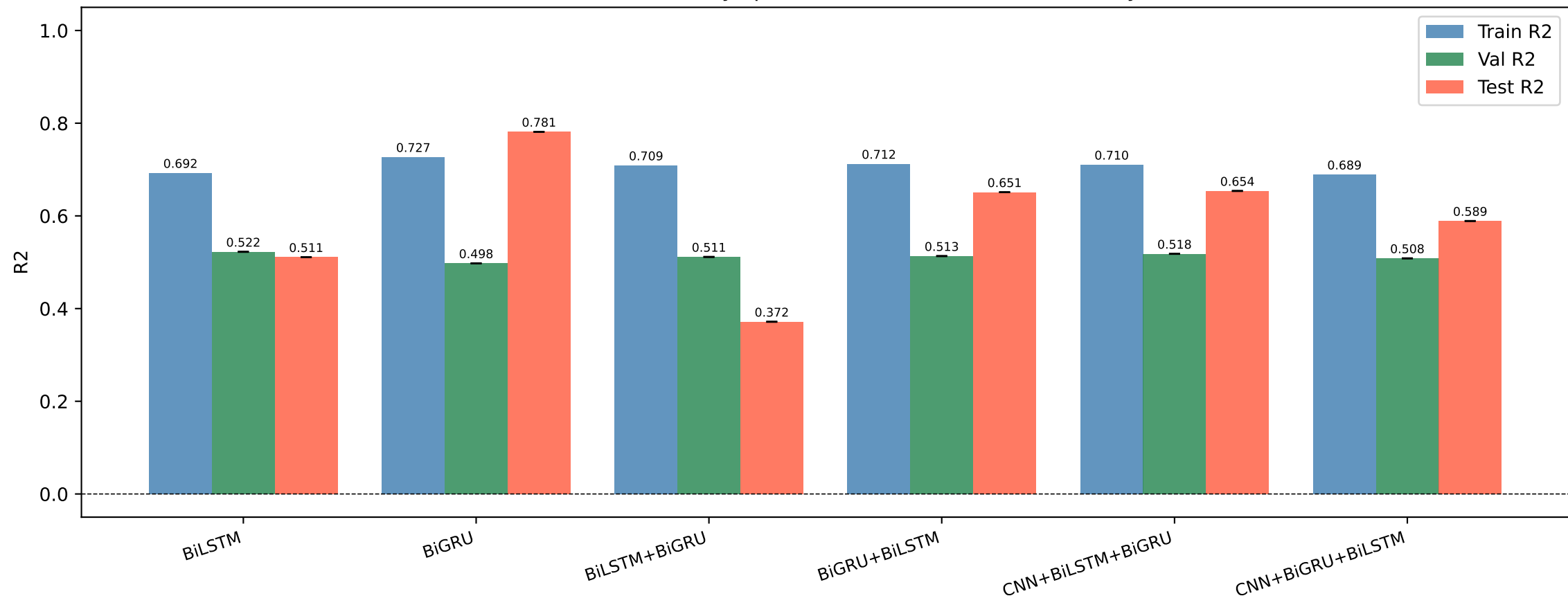
Bashundhara - R2 by split (model selection uses VAL only)
