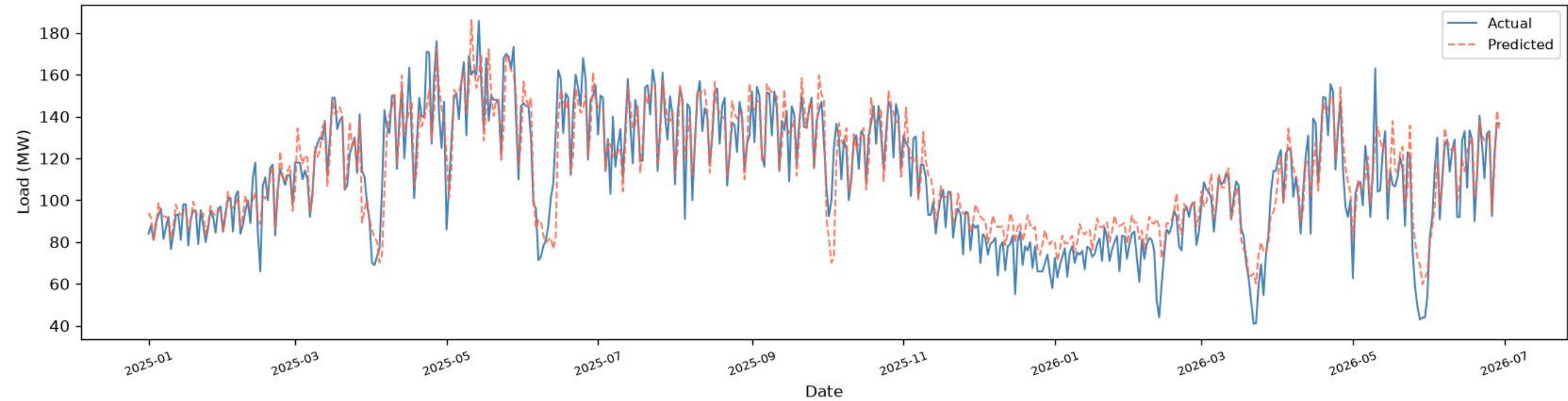
Dhanmondi | BiGRU+BiLSTM - TEST ( \geq 2025 ), one-day-ahead ( R^2=0.8411 , RMSE=11.73 , MAE=8.75 , n=536 )
