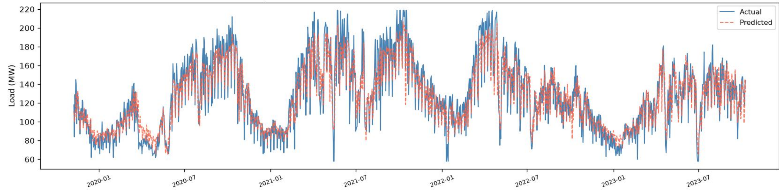
Dhanmondi | BiGRU+BiLSTM - TRAIN (fit block) (R2=0.8670, RMSE=13.72, MAE=10.23, n=1395)
