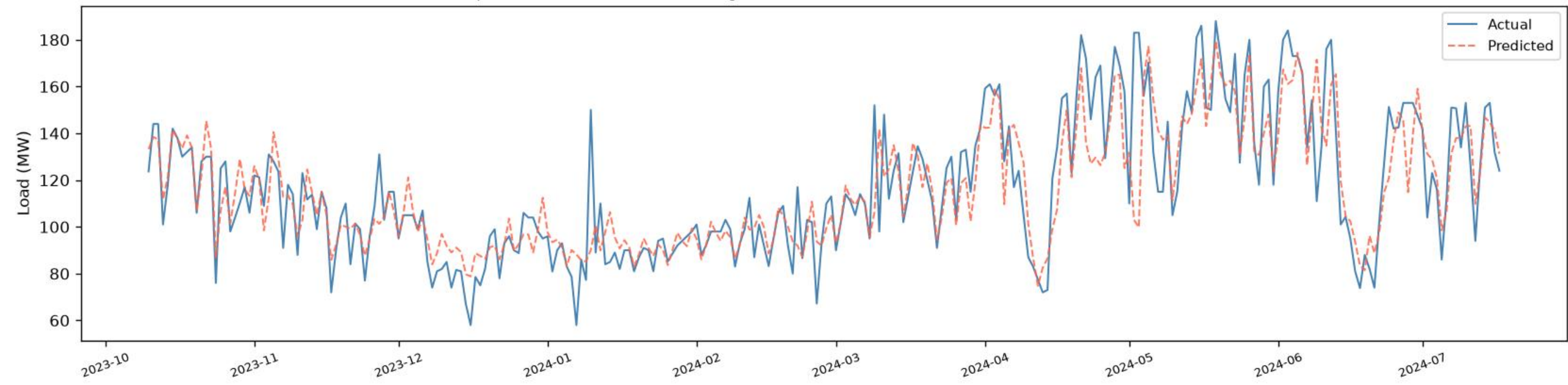
Dhanmondi | BiGRU - VALIDATION (chronological, before test) (R2=0.7319, RMSE=15.42, MAE=10.47, n=271)
