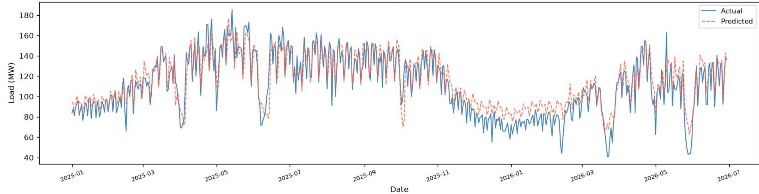
Dhanmondi | BiLSTM+BiGRU - TEST ( \geq 2025 ), one-day-ahead ( R^2=0.8174 , RMSE=12.57 , MAE=9.72 , n=536 )
