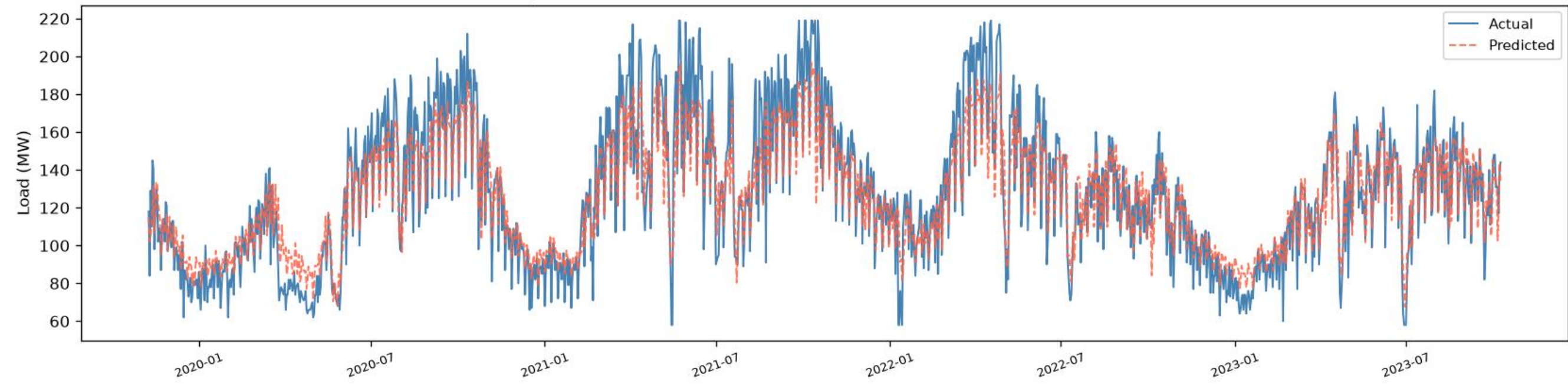
Dhanmondi | BiLSTM+BiGRU - TRAIN (fit block) (R2=0.8387, RMSE=15.11, MAE=11.50, n=1395)
