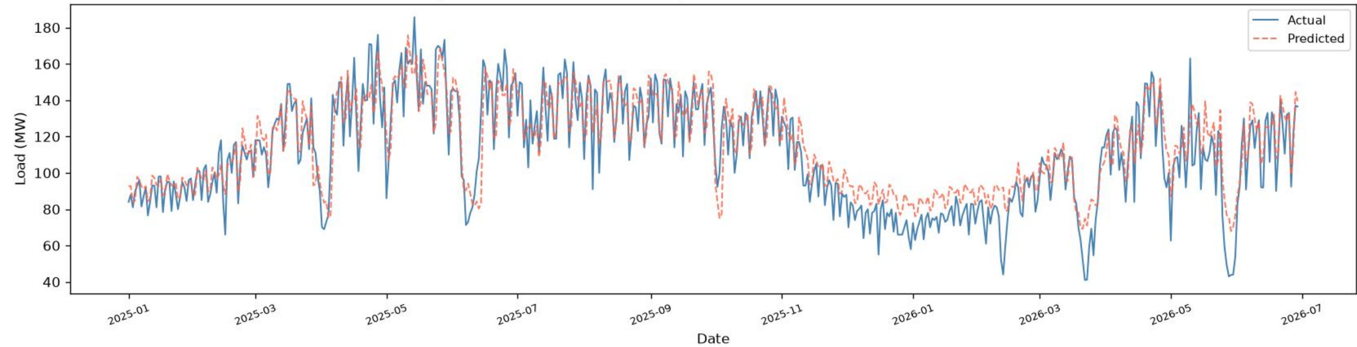
Dhanmondi | BiLSTM - TEST ( \geq 2025 ), one-day-ahead ( R^2=0.8078 , RMSE=12.89 , MAE=9.93 , n=536 )
