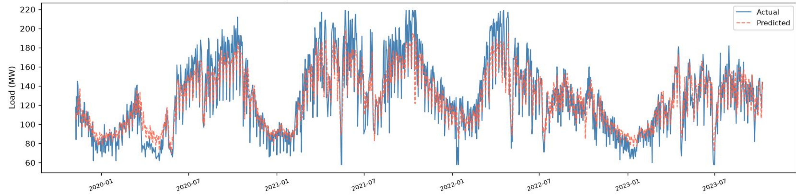
Dhanmondi | BiLSTM - TRAIN (fit block) ( R^2=0.8317 , RMSE=15.43, MAE=11.89, n=1395)
