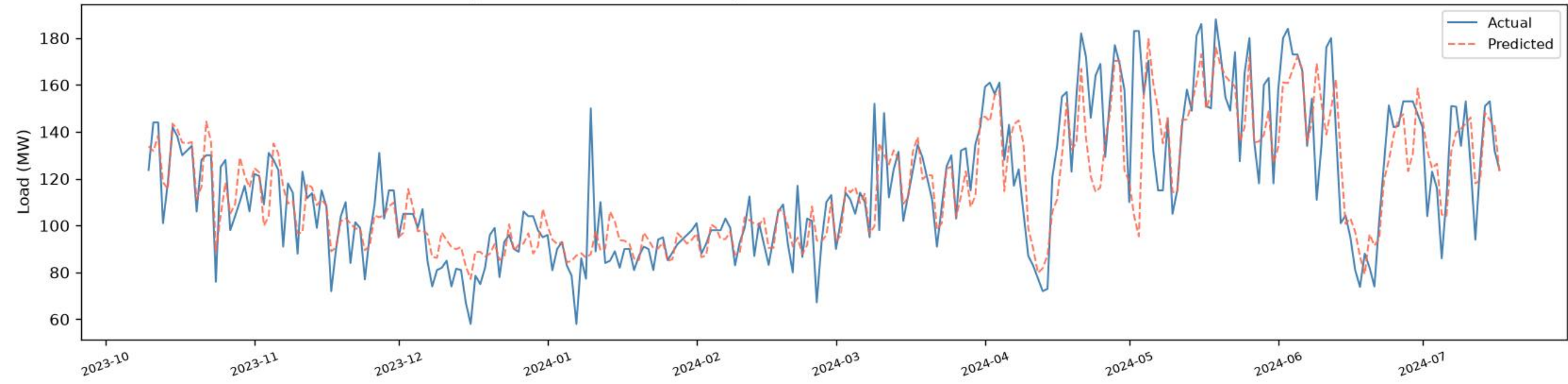
Dhanmondi | BiLSTM - VALIDATION (chronological, before test) ( R^2=0.7001 , RMSE=16.30, MAE=11.21, n=271 )
