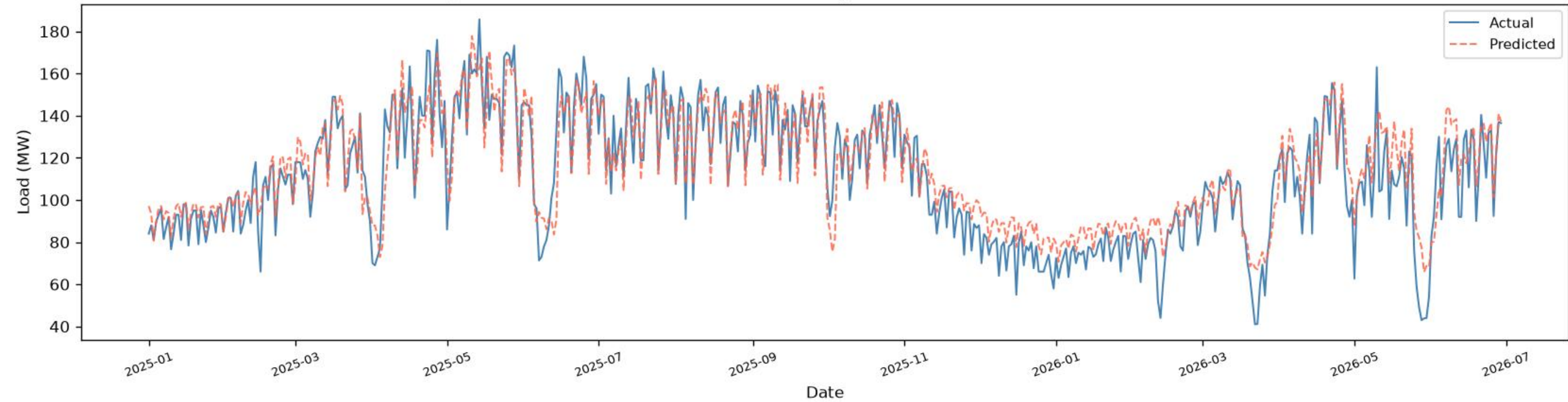
Dhanmondi | CNN+BiGRU+BiLSTM - TEST ( \geq 2025 ), one-day-ahead ( R^2=0.8425 , RMSE=11.67 , MAE=8.99 , n=536 )
