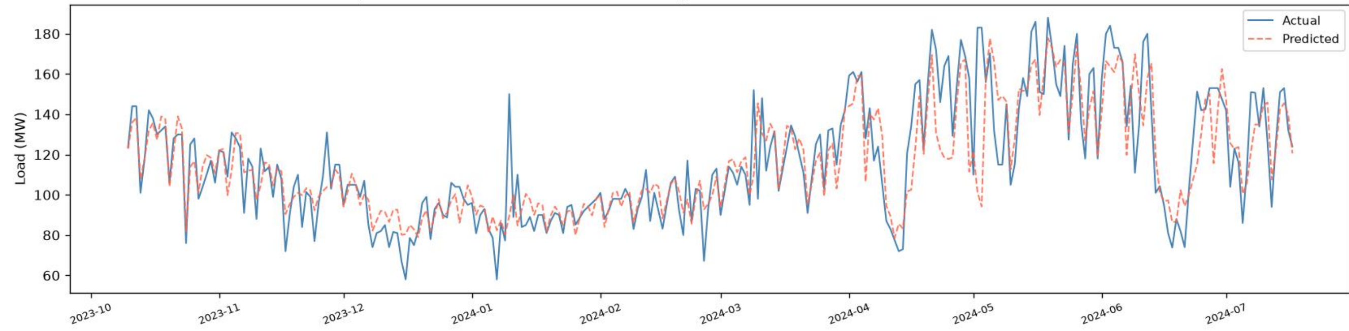
Dhanmondi | CNN+BiGRU+BiLSTM - VALIDATION (chronological, before test) ( R^2=0.7129 , RMSE=15.95 , MAE=10.46 , n=271 )
