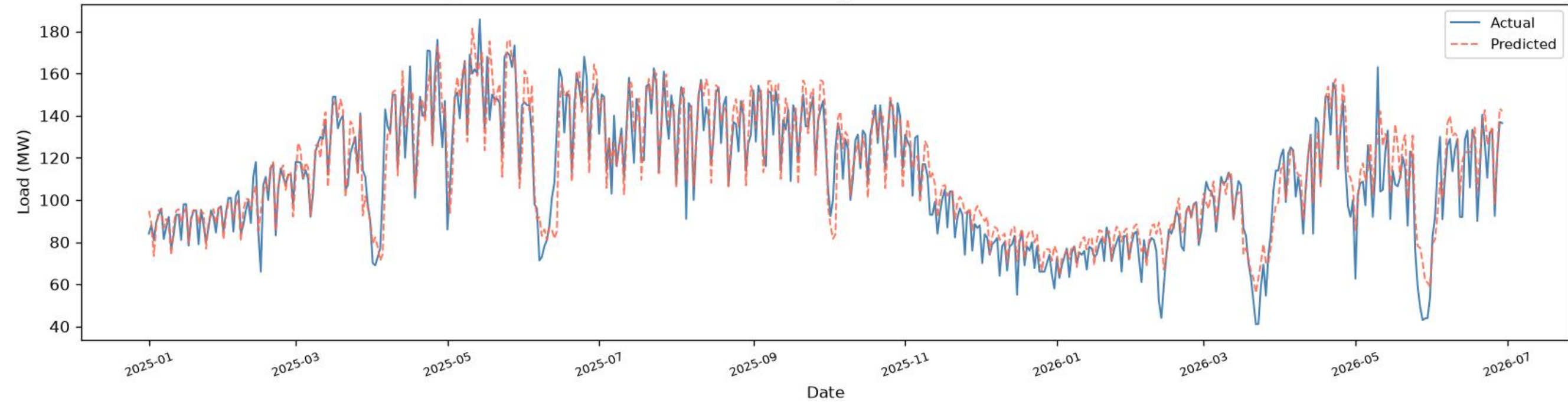
Dhanmondi | CNN+BiLSTM+BiGRU - TEST ( \geq 2025 ), one-day-ahead ( R^2=0.8717 , RMSE=10.54 , MAE=7.67 , n=536 )
