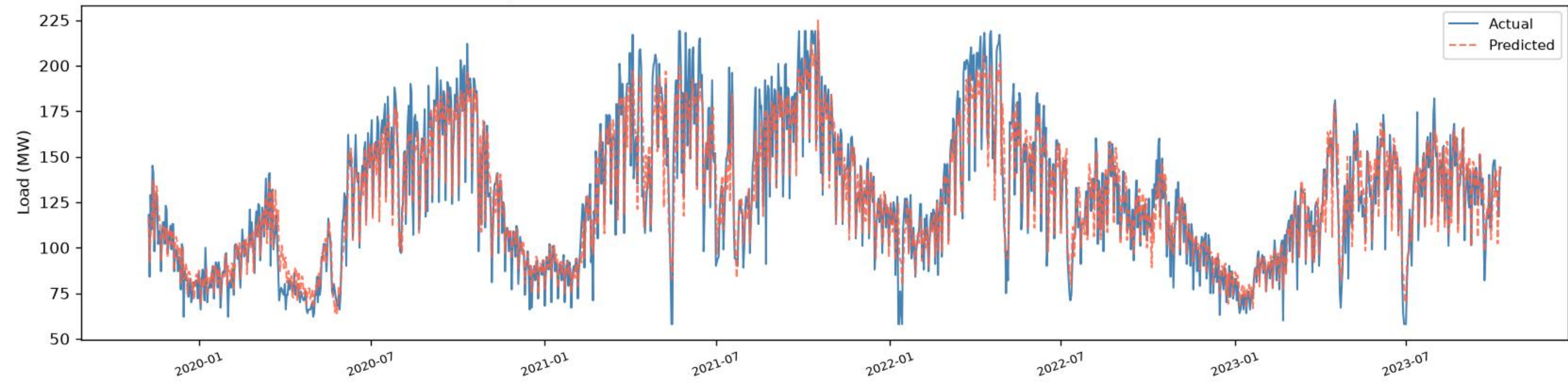
Dhanmondi | CNN+BiLSTM+BiGRU - TRAIN (fit block) (R2=0.9008, RMSE=11.85, MAE=8.53, n=1395)
