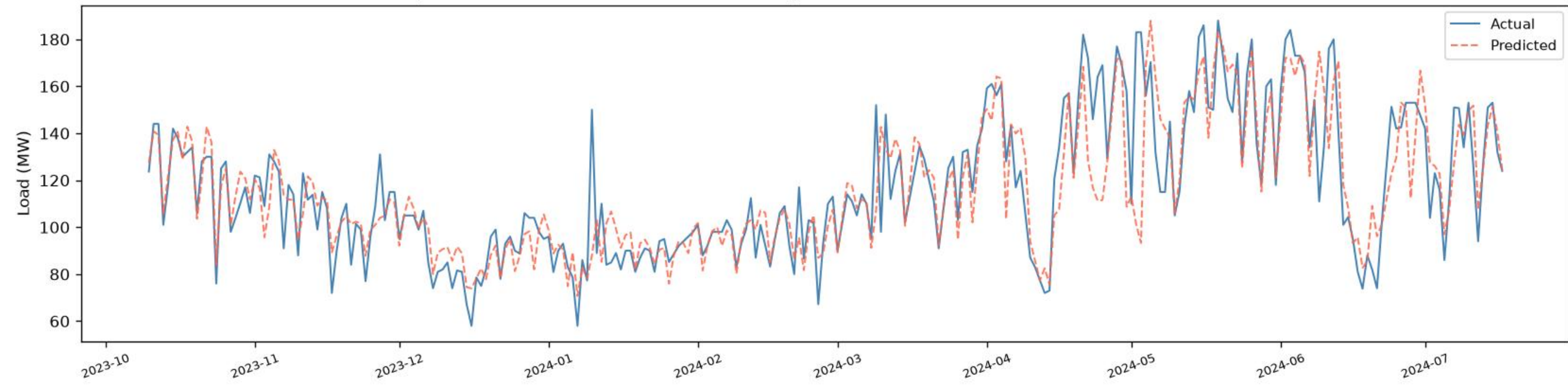
Dhanmondi | CNN+BiLSTM+BiGRU - VALIDATION (chronological, before test) ( R^2=0.7135 , RMSE=15.94 , MAE=10.08 , n=271 )
