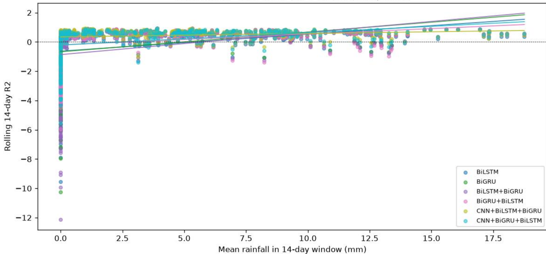
Dhanmondi - Rain vs R2 (all 6 models, test period)
